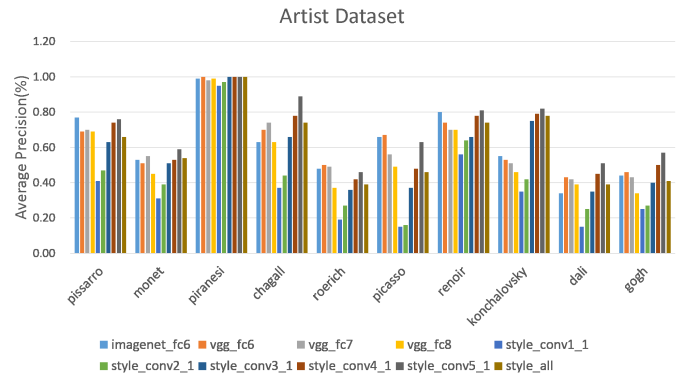
Figure 6: All per-category APs on “Artist dataset”.
