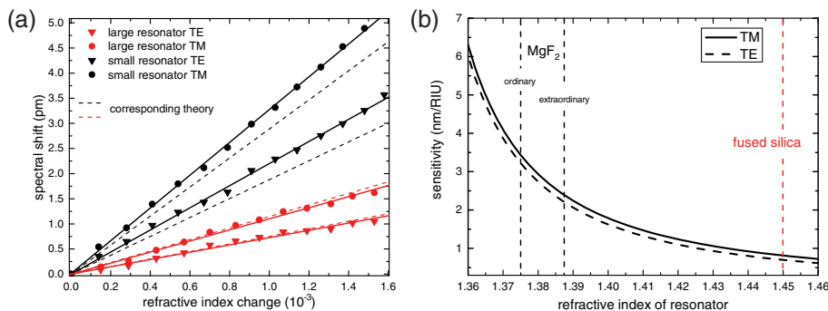
(a) Resonance shift of a R = 2.91 mm and R = 1.19 mm crystalline WGM resonator upon variation of the bulk refractive index of the surrounding medium (water), as controlled by adding glycerol of differing concentration. (b) Bulk sensitivity of WGM refractometers as a function of resonator refractive index [cf. Eq. (5)], based on a 2 mm resonator in water operating at 795 nm. Reprinted with permission from [142]. Copyright 2014 Optical Society of America.
