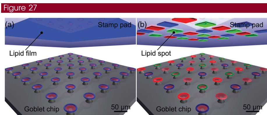
Schematic of stamp pad technique for parallel functionalization of goblet resonators. (a) Large-scale uniform surface functionalization. (b) Multiplexed surface functionalization using an array of phospholipids with different functional head groups [49]. Copyright Wiley-VCH Verlag GmbH & Co. KGaA. Reproduced with permission.
