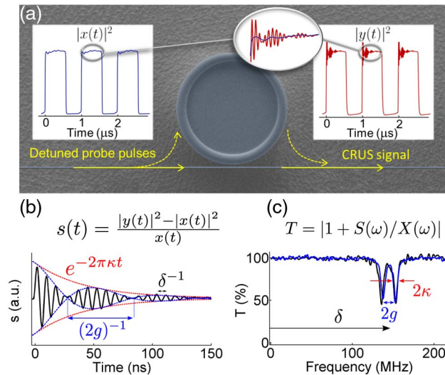
(a) Schematic of cavity ring-up spectroscopy (CRUS) with a WGM resonator. (b) Typical example of the ring-up signal. (c) Fourier transform of the ring-up signal, from which the WGM spectrum is recovered. In this case a split mode is seen. Reprinted from [232].
