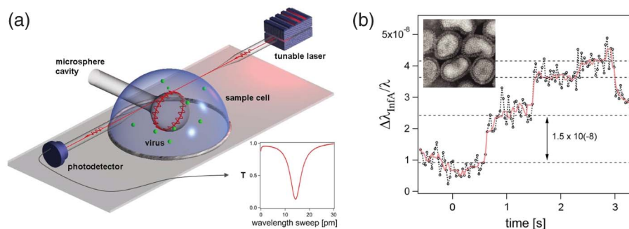
(a) Schematic of WGM biosensor with transmission spectrum. (b) Steps in resonance frequency observed upon binding of individual Influenza A virions (inset). Adapted from [149] [Copyright (2008) National Academy of Sciences, U.S.A.].
