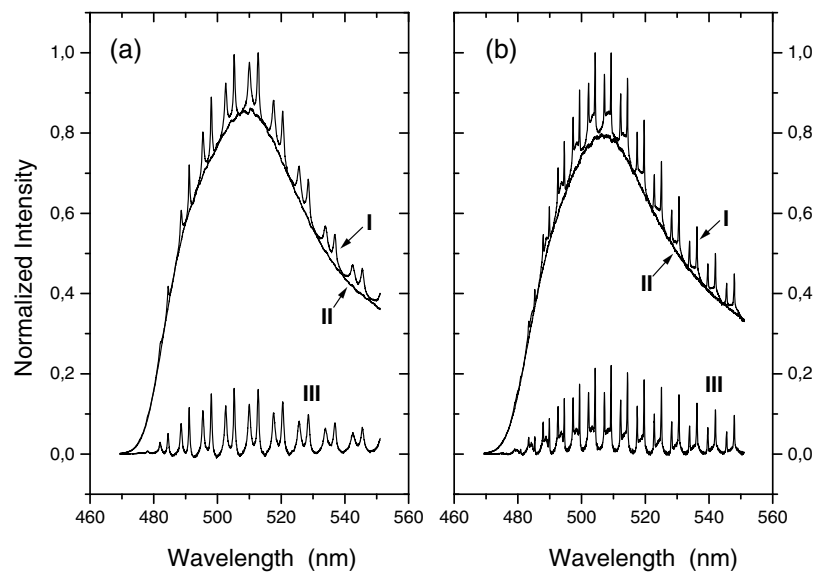
Fluorescence emission of dye-doped polystyrene beads of (a) \sim 8 \mu\text{m} and (b) 10 \mu\text{m} in diameter, respectively, immersed in water, exhibiting WGM excitations (line I). Line II shows the fluorescence emission of odd-shaped particles that do not support WGMs. Line III shows the difference spectra of (I) and (II). Reprinted from [309]. Copyright 2014 The EPJ Publishing Consortium. With kind permission of The European Physical Journal (EPJ).
