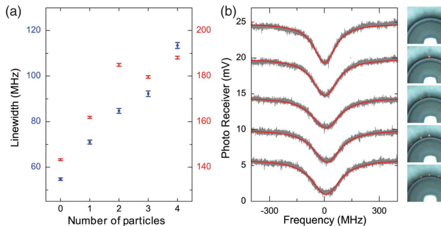
(a) Mode broadening induced in two resonant WGMs upon binding of 70-nm-radius polystyrene nanoparticles. (b) Experimental transmission spectrum for 0 (top) to 4 (bottom) bound polystyrene nanoparticles with the corresponding enhanced optical images of the toroidal microcavity. Reprinted from [182].
