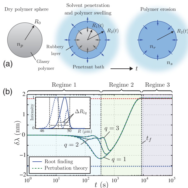
(a) Schematic of penetrant dynamics upon introduction of a glassy polymer microsphere into a solvent bath. Arrows depict the direction of movement of the polymer interfaces. (b) Temporal evolution of resonance wavelength shift \delta\lambda for polystyrene–water polymer-penetrant system. Inset shows radial extent of WGM in an unperturbed 50\ \mu\text{m} polystyrene microsphere. Reprinted from [172].
