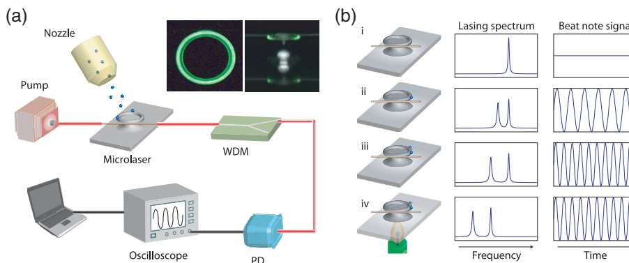
(a) Experimental schematic for nanoparticle detection based on mode splitting of a WGM microlaser. (b) Surface deposition of nanoparticles induces mode splitting in the laser spectrum that can be detected via a heterodyned beat note. Reprinted with permission from [219]. Copyright 2011.
