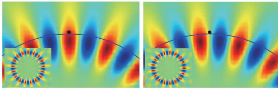
Intensity profiles of the symmetric (left) and antisymmetric (right) normal modes created via nanoparticle backscattering. Reprinted with permission from [185].
