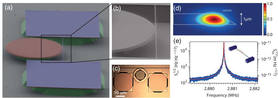
(a) Scanning electron microscopy image of the hybrid optomechanical force sensor, with (b) zoom in of the coupling region. (c) Optical micrograph of the tapered fiber used to couple and read out from the system. (d) FEM simulation of the mode distribution in the resonator near the nanobeam. (e) Mechanical resonance of the nanobeam. Reprinted with permission from [18]. Copyright 2012.
