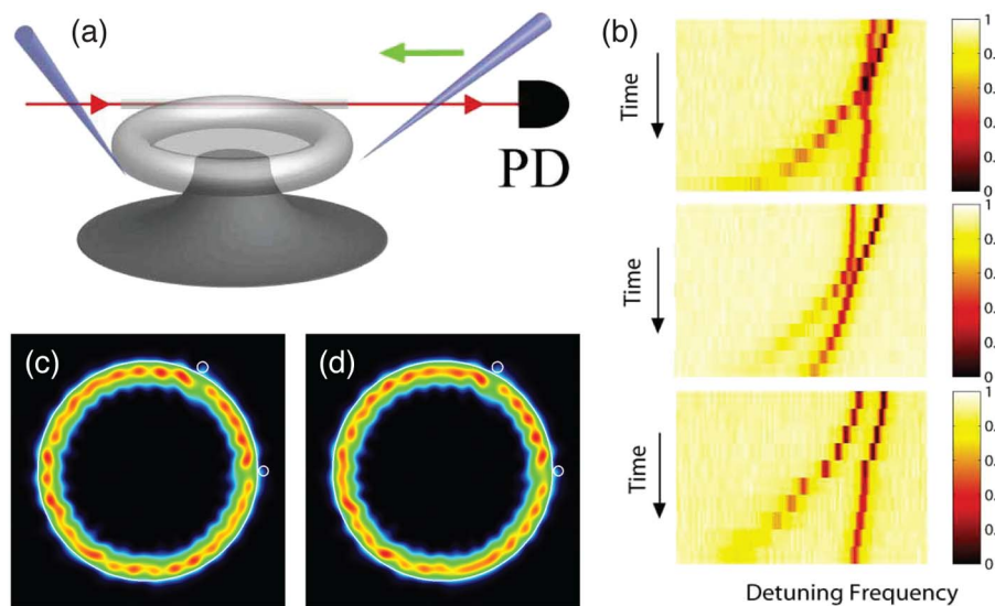
(a) Schematic of experimental setup, allowing controlled manipulation of mode splitting via positioning of two nano-probes near a toroidal WGM resonator. (b) Spectral intensity as a function of tip size, which was varied with time, showing mode crossing (top), anticrossing (middle), and shift (bottom) as arising from different tip placements. Reprinted with permission from [196]. Copyright 2010 Optical Society of America. (c) and (d) show simulated eigenmode intensity profiles for two scatterers positioned near a microcavity sensor such that the sensor operates close to an exceptional point. Reprinted with permission from [214]. Copyright 2014 by the American Physical Society.
