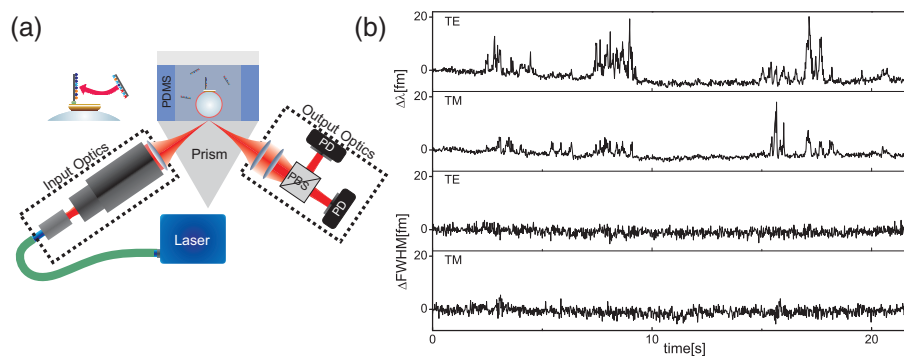
(a) Prism-based microcavity biosensing setup. (b) Single nucleic acid interactions with a nanorod-enhanced WGM sensor. Data show different transient events for TE and TM modes, and negligible change in the linewidth due to a purely reactive effect on the WGMs. Adapted with permission from [4]. Copyright 2014.
