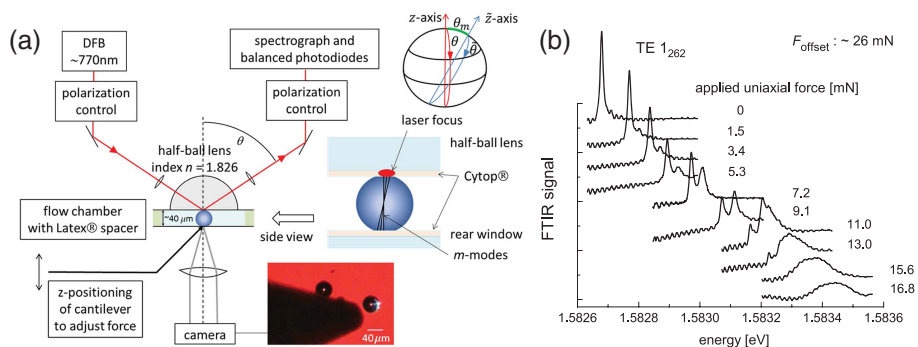
(a) Experimental scheme for application of a uniaxial pressure to a polystyrene sphere by means of a cantilever. (b) FTIR spectra showing the induced mode shift and splitting upon application of forces of increasing strength. Reprinted with permission from [175]. Copyright 2013, AIP Publishing LLC.
