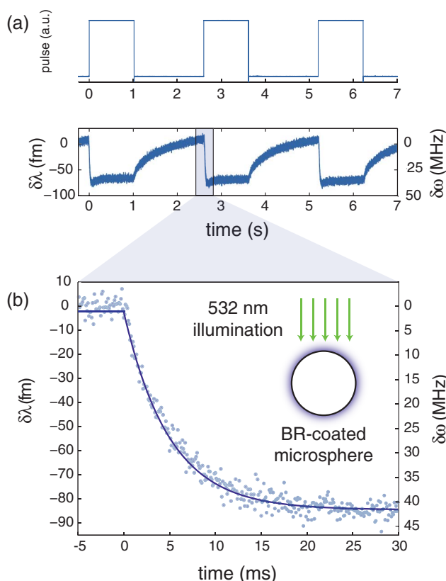
Measurement of conformational changes in BR. (a) 532 nm pulse scheme used for measurement and corresponding light-induced frequency shifts. (b) The initial conformational change occurs with a time constant of 5 ms.
