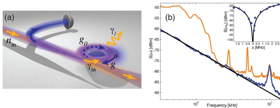
(a) Illustration of the backscatter-based detection scheme. (b) Frequency noise power spectra for frequency shift (light orange) and backscatter measurements (dark blue). Black line represents a 1/f^2 fit to the backscatter data. Inset shows the backscattered power spectrum at the modulation frequency as a function of the detuning. Reprinted from [170].
