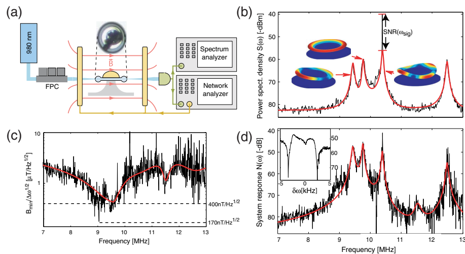
(a) Experimental setup showing a WGM resonator with a Terfenol-D sample attached. (b) Brownian noise spectrum with magnetic excitation at 10.38 MHz. (c) Magnetic-field sensitivity as a function of frequency. (d) System response as a function of applied magnetic-field frequency. Inset: magnified system response centered around 10.385 MHz. Reprinted from [16].
