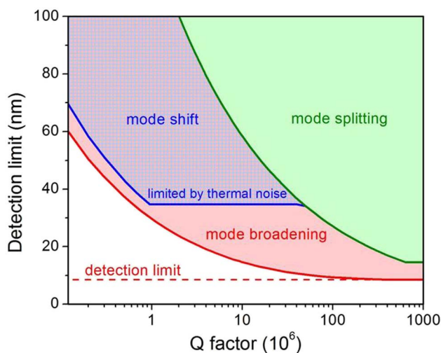
Comparison of the theoretical detection limit for spherical polystyrene nanoparticles in air using different WGM detection modalities: resonance shifts (blue), mode broadening (red), and mode splitting (green). Reprinted from [182].
