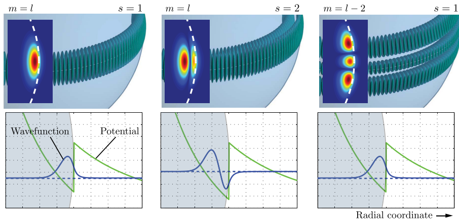
(Top) Iso-intensity surfaces and intensity cross sections (inset) for (left) fundamental TE mode l = m , (middle) second-order radial mode s = 2 , and (right) azimuthal mode m = l - 2 in a spherical resonator. (Bottom) Effective potentials and radial wavefunctions for the same WGMs as in the top row.
