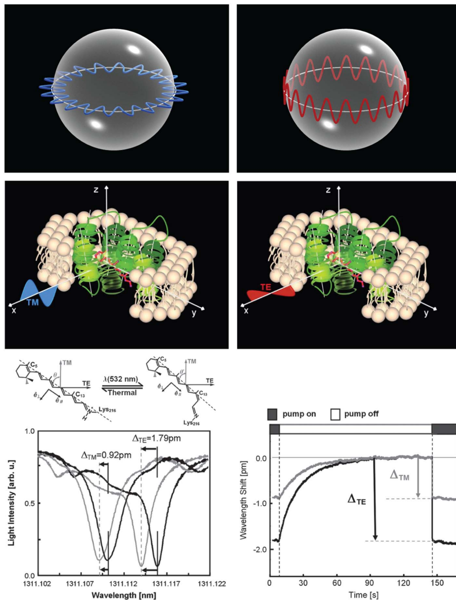
(Top) Schematic of TM (left) and TE (right) WGMs in a dielectric microsphere. (Middle) Three-dimensional ribbon model of seven transmembrane \alpha helices representing the structure of bacteriorhodopsin embedded in a lipid bilayer with a covalently bound chromophore. (Bottom) Transmission spectra for TM and TE WGMs, showing a resonance shift upon photoexcitation of the adsorbed bacteriorhodopsin (left) and dynamics of a photoinduced transformation observed by tracking TM and TE WGMs (right). Adapted from [192].
