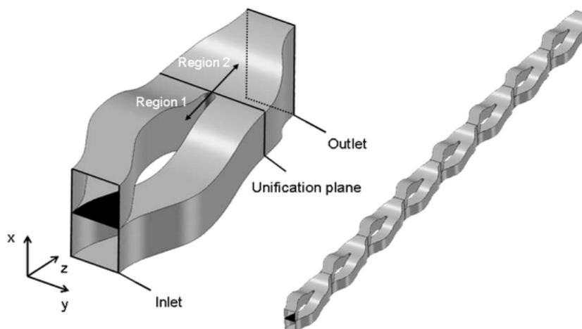
Figure 18. Enlarged view of the SAR unit (left) composing the 8-unit mixer (from Hardt et al. [35]).
