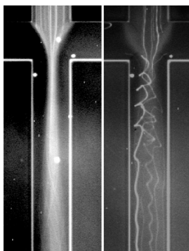
Figure 25. Particle trajectories with static (left-hand-side photo) and time-varying (right-hand-side photo) electric fields at the inlet of the channel (from Shin et al. [47]).
