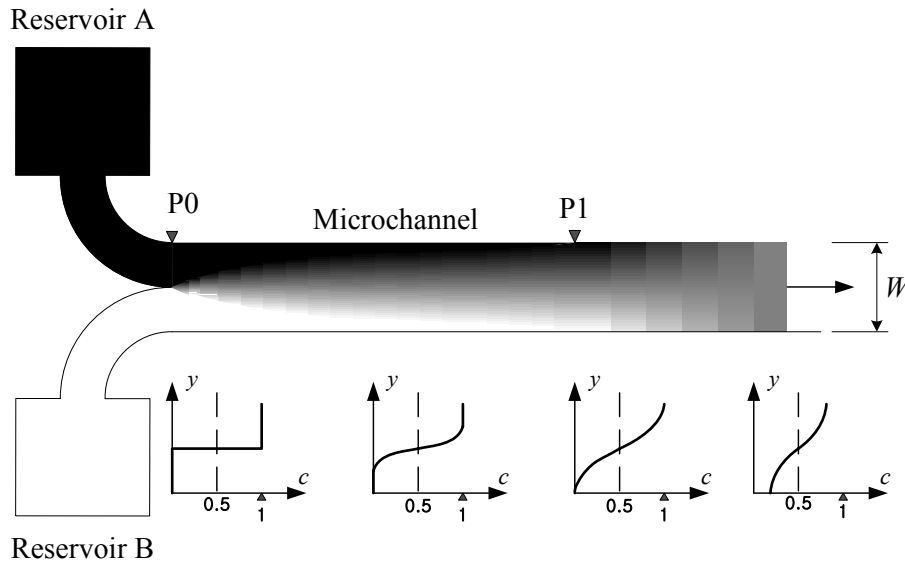
Figure 2. Schematic of a typical concentration distribution (grey level) within a microchannel without a specific mixing element. The graphs below show the concentration distribution as a function of the coordinate normal to the channel wall, y , at several channel sections.
