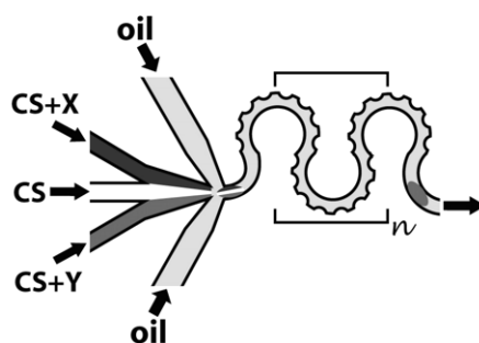
Figure 26. A meandering channel with bumps on the outer side for use in mixing three kinds of liquids (from Liau et al. [49]).
