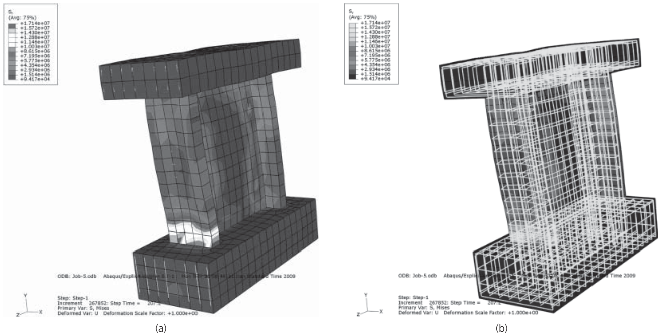
Figure 13. (a) Stress of SW4 under revised cyclic loading. (b) Stress of SW4 with steel reinforcing detail under revised cyclic loading
