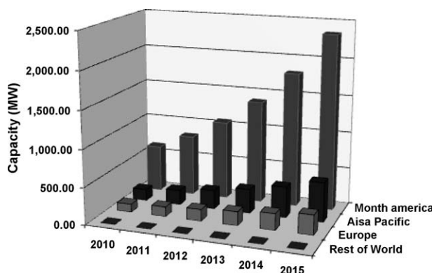
Figure 5: 2009 Microgrid Forecast: 2010–2015
