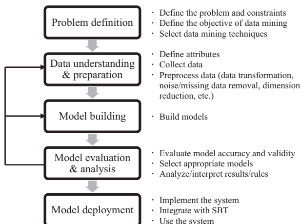
Fig. 2. The data mining methodology.
