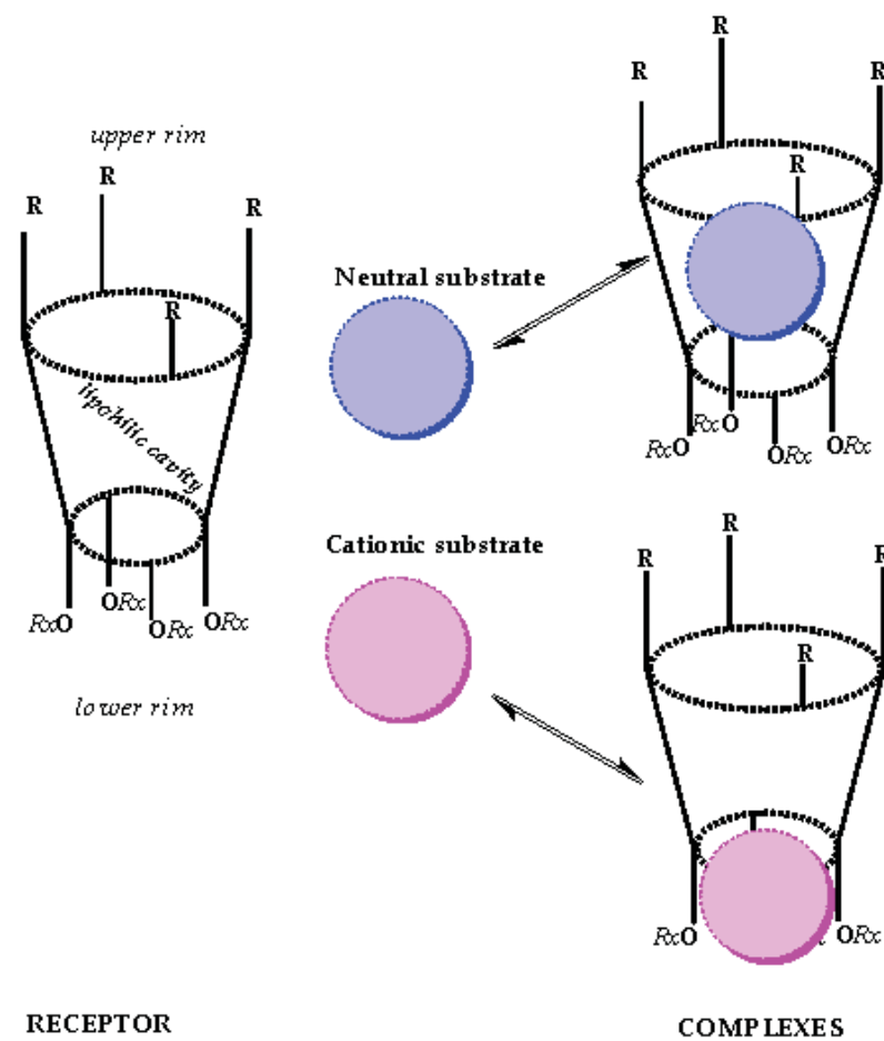
Fig. 3. Schematic representation of calixarene complexation with neutral and cationic substrates.
