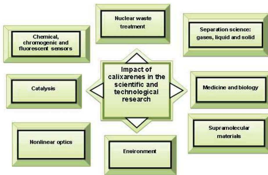
Fig. 1. Applications for calixarenes in science and technology.
