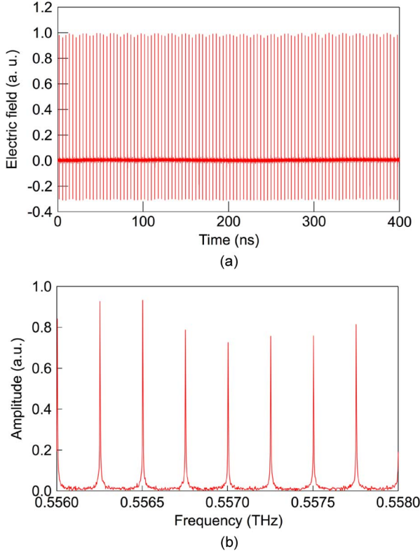
Fig. 4. (a) Temporal waveform of electric field in 100 consecutive THz pulses (time window = 400 ns). (b) Amplitude spectrum of THz comb mode around 0.557 THz.
