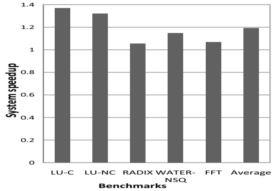
Figure 12. System speedup
